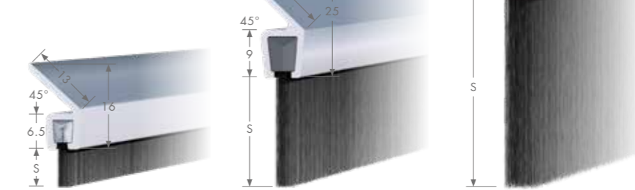
Y-Profile (scale 1:1)
